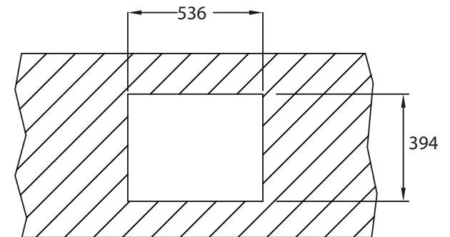
Hueco para bajo encimera Fitting hole for undermounted sink
